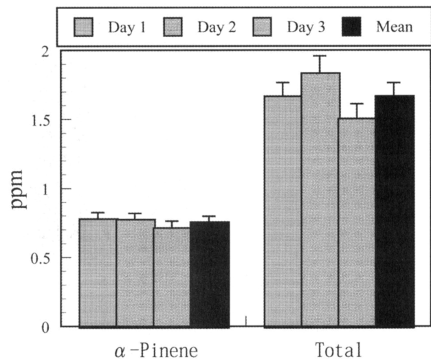
Fig. 1. Concentrations of \alpha -pinene and the total phytoncides in the hotel room air. Data are presented as the mean+SE (n=12).
